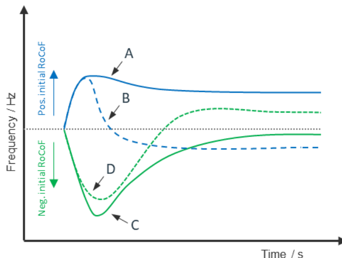
Figure 7 – Illustration of 4 time-domain trajectory cases
