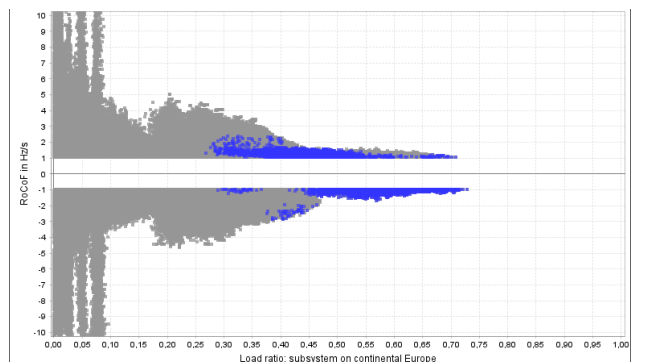
Figure 11 – Subset of total blackout cases due to both areas experiencing an absolute RoCoF value greater than 1 Hz/s after additional kinetic energy in the simplified example.
