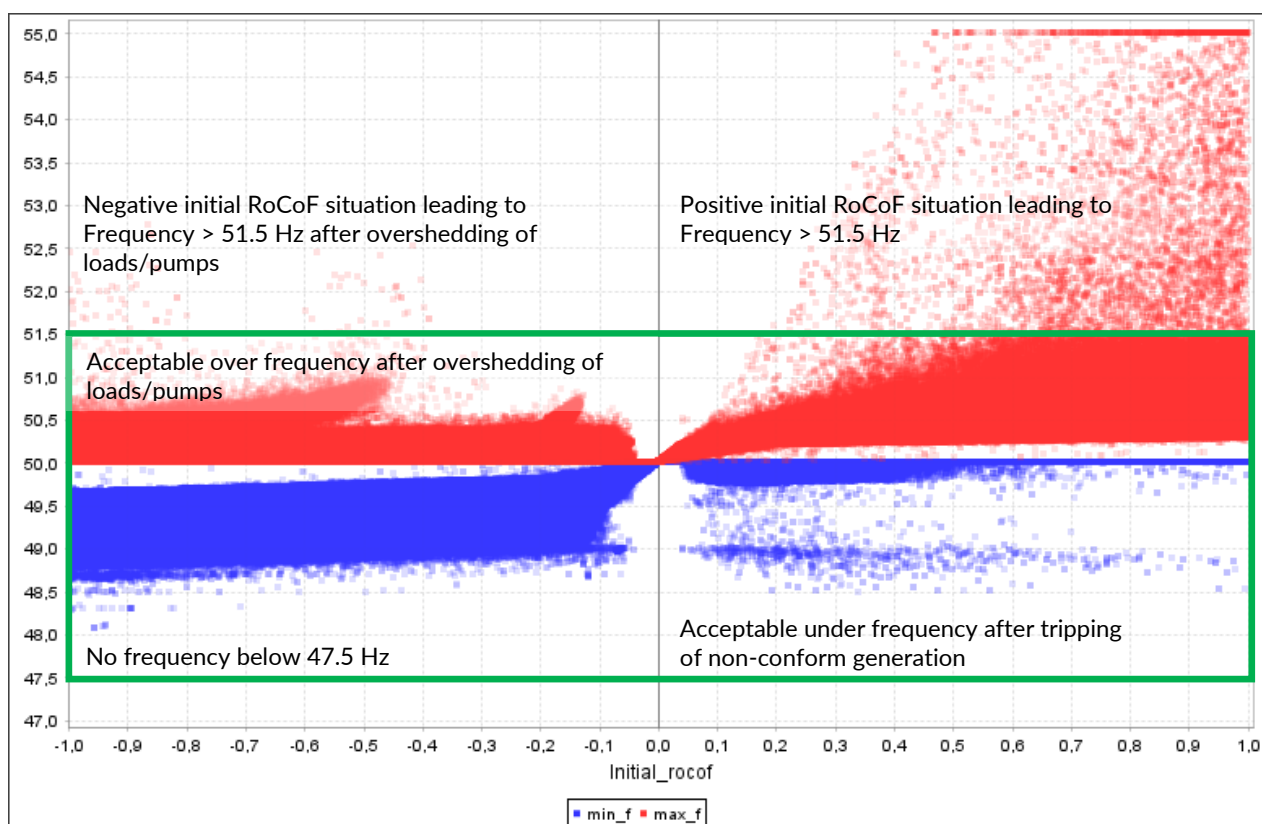
Figure 6 – DE 2040: all cases with a |\text{RoCoF}| < 1 \text{ Hz/s} with load self-regulation of 2%, 200ms load shedding delay and a generalized LFDD scheme with 6 stages (49.0 Hz: 5 %, 48.8 Hz: 8 %, 48.6 Hz: 8 %, 48.4 Hz: 8 %, 48.2 Hz: 8 %, 48.0 Hz: 8 %).
