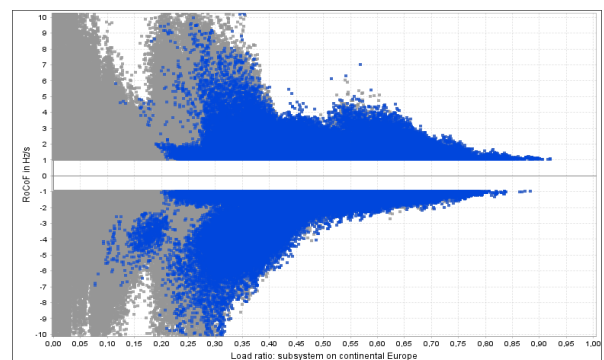
Figure 4 – Subset of total blackout cases due to both areas experiencing an absolute RoCoF value greater than 1 Hz/s |\text{RoCoF}| values above 1 Hz/s for each subsystem of the CE SA (consisting of two subsystems per split combination) plotted against the load ratio of each subsystem with regard to the CE SA for the different TYNDP 2022 scenarios (each dot represents an hour and split combination): NT 2030, NT 2040 – National Trends 2030, 2040; DE 2030, DE 2040 – Distributed Energy 2030, 2040; GA 2030, GA 2040 – Global Ambition 2030, 2040. Values above 10 Hz/s, appearing for small ratios only, are not shown.
