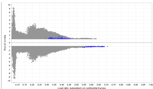
Figure 11 – Subset of total blackout cases due to both areas experiencing an absolute RoCoF value greater than 1 Hz/s after additional kinetic energy in the simplified example.
