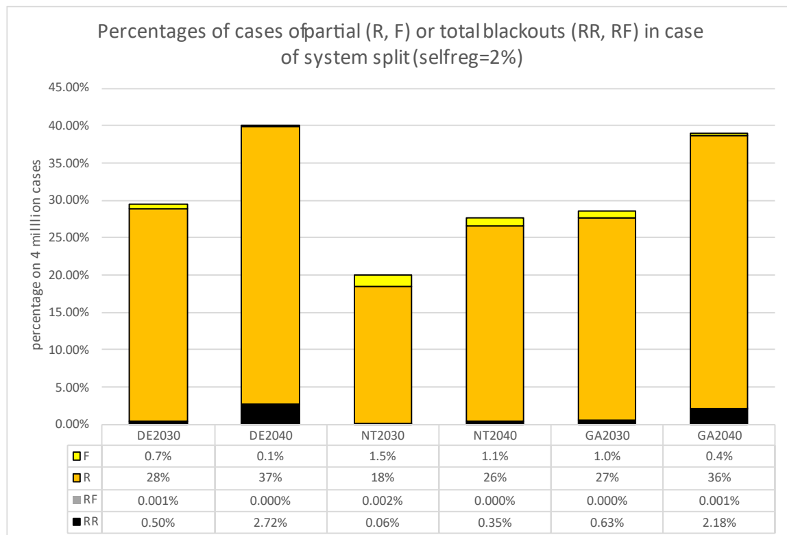
Figure 5 – Percentages of cases of partial or total blackouts in the event of system split.
