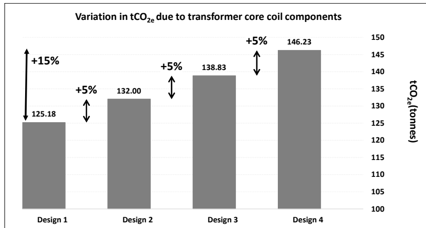
Figure 5. Impact of transformer loss specification: core and coil carbon footprint
