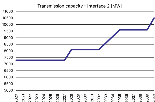
Figure 8. Planned capacity development for Interface 2, the boundary between bidding zones SE2 and SE3.
